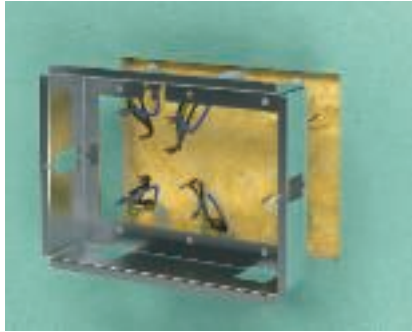
Mounting of cavity wall support Insert the cavity wall support in the prepared mounting opening.
