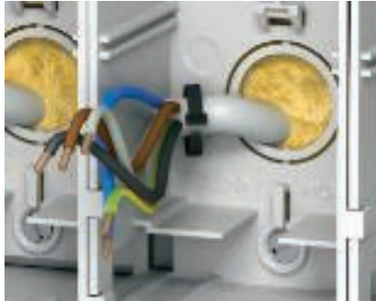
Cable strain relief device Pull the installation cables through the cable gland and relieve the strain on the housing base.
