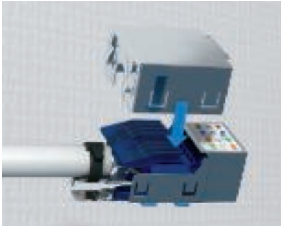
Device connection - Mounting shield hood The shield hood is placed on the connection module from the top and engaged. The shield hood is only used for shielded connection modules.
